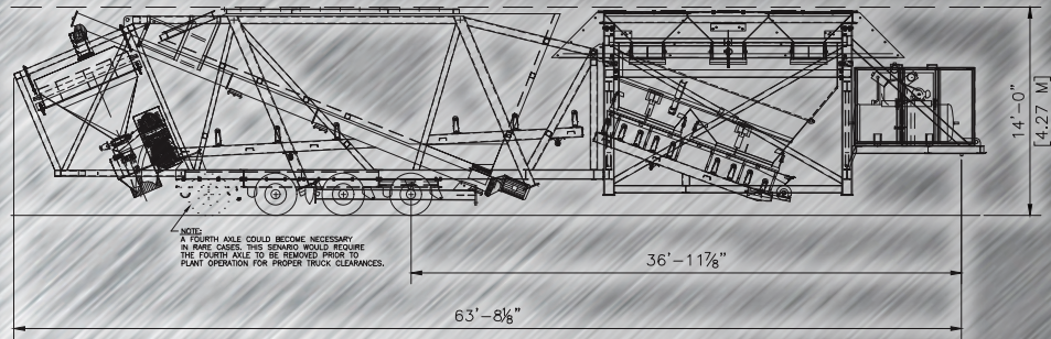
EAGLE MOBILE - TOWING POSITION
