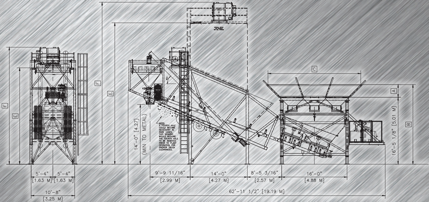
EAGLE MOBILE - TOWING POSITION
